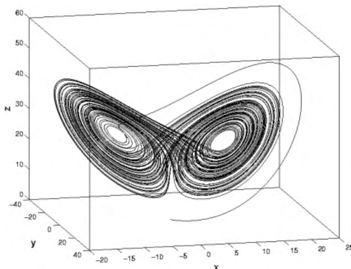
FIG. 2: Representation of a Lorentz attractor region
